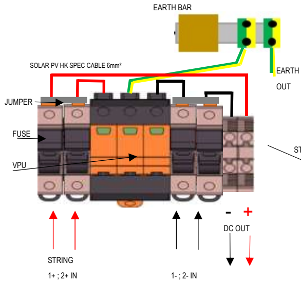
WIRING ARRANGEMENT
